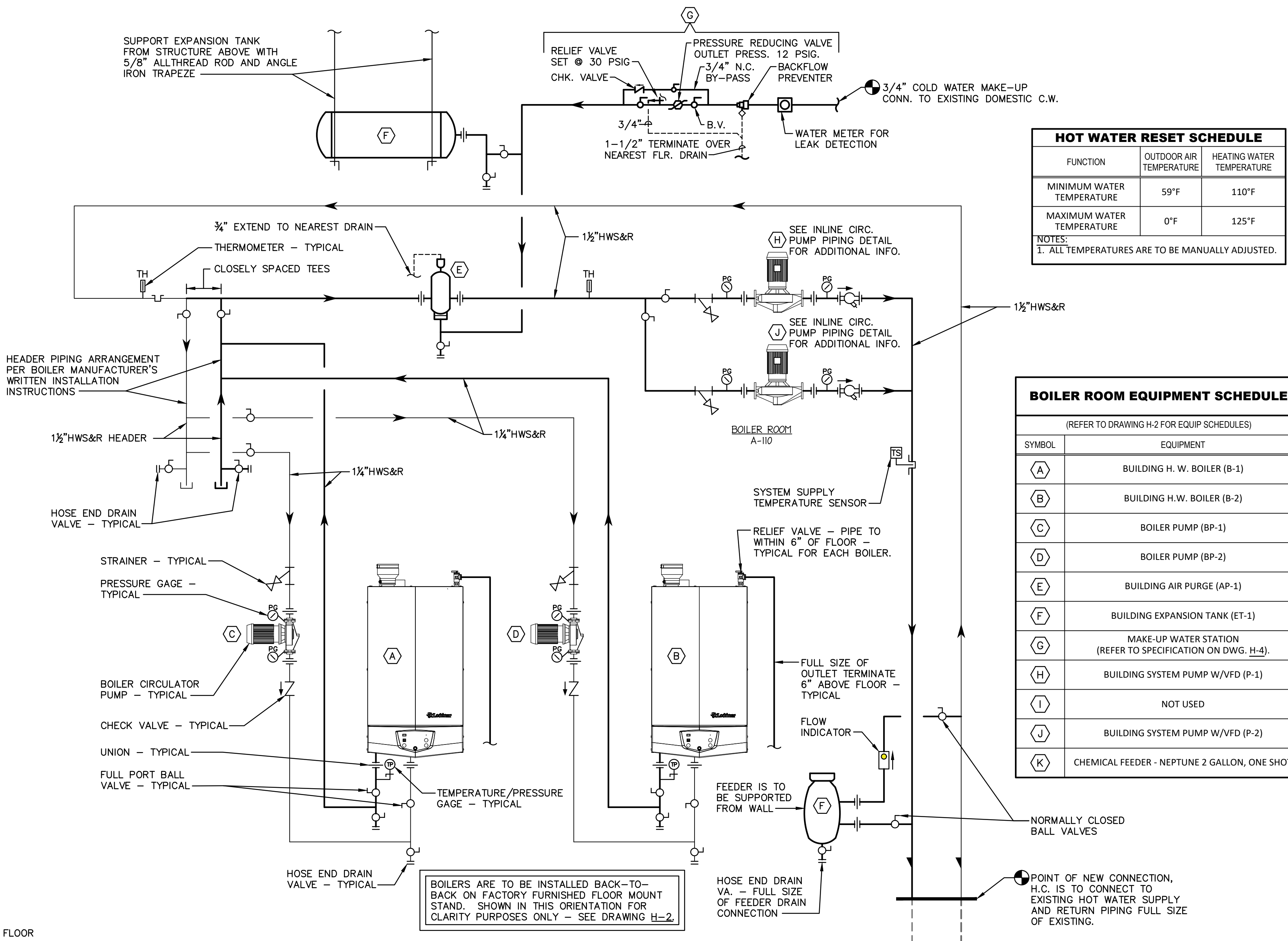
BOILER ROOM SCHEMATIC FLOW DIAGRAM NOT TO SCALE
